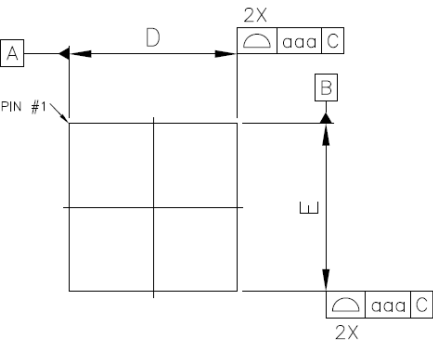
Figure 68: Top View
