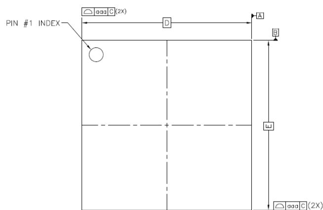
Figure 64: Top View
