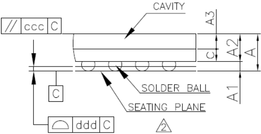
Figure 70: Side View
