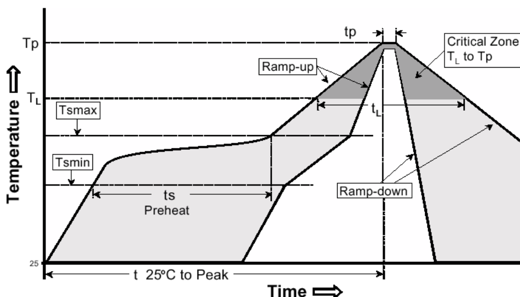
Figure 75: Reflow Condition
