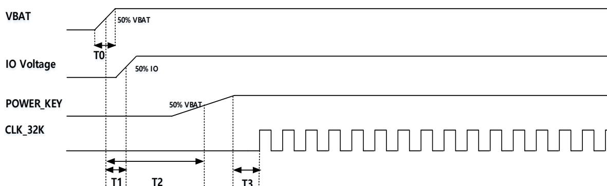
Figure 11: Power On Sequence
