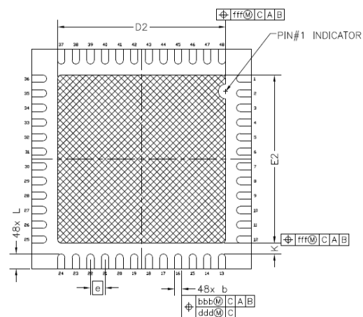
Figure 65: Bottom View
