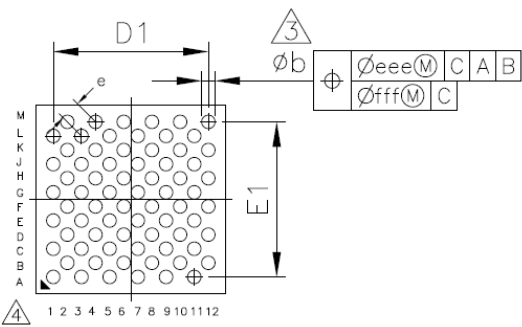
Figure 69: Bottom View
